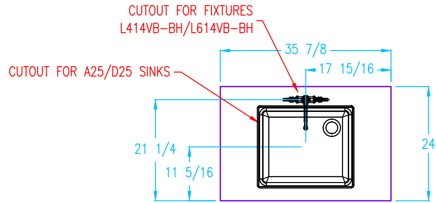
1" THICK EPOXY TOP LEFT & RIGHT EDGES NOT FINISHED. FRONT EDGE IS FINISHED.
